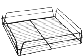
GLASS BASKET PVC Coated Length | 355mm Width | 355mm Height | 75mm Colour | Black
