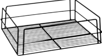
GLASS BASKET PVC Coated Length | 435mm Width | 355mm Height | 125mm Colour | Black
