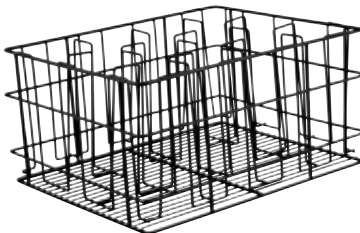
12 COMPARTMENT BASKET PVC Coated Compartment Size: 110 x 105mm Length | 430mm Width | 355mm Height | 215mm Colour | Black
