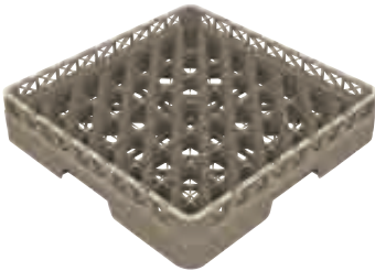
49 COMPARTMENT BASKET Maximum Glass Diameter 63mm Length | 500mm Width | 500mm Height | 80mm
