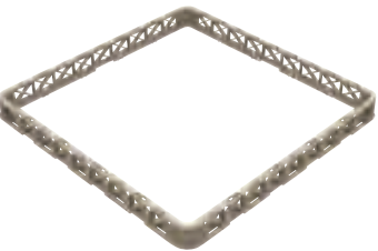
OPEN EXTENDER Length | 500mm Width | 500mm Height | 40mm
