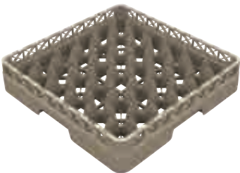
36 COMPARTMENT BASKET Maximum Glass Diameter 73mm Length | 500mm Width | 500mm Height | 80mm
