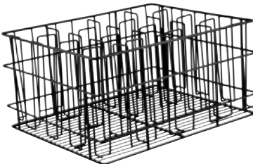
16 COMPARTMENT BASKET PVC Coated Compartment Size: 105 x 75mm Length | 430mm Width | 355mm Height | 215mm Colour | Black
