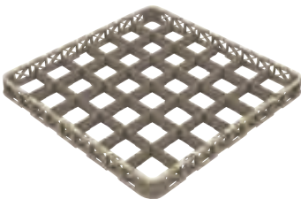
36 COMPARTMENT EXTENDER Maximum Glass Diameter 73mm Length | 500mm Width | 500mm Height | 40mm
