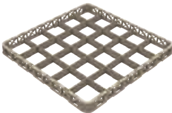
25 COMPARTMENT EXTENDER Maximum Glass Diameter 89mm Length | 500mm Width | 500mm Height | 40mm
