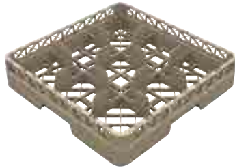
9 COMPARTMENT BASKET Maximum Glass Diameter 151mm Length | 500mm Width | 500mm Height | 80mm
