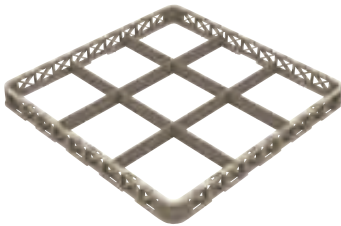
9 COMPARTMENT EXTENDER Maximum Glass Diameter 151mm Length | 500mm Width | 500mm Height | 40mm
